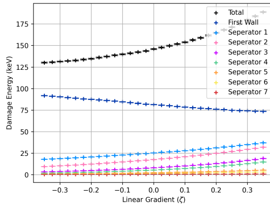
Figure C2: Total damage energy deposited into the plasma-facing FW and internal structural separators across the geometric gradient.
