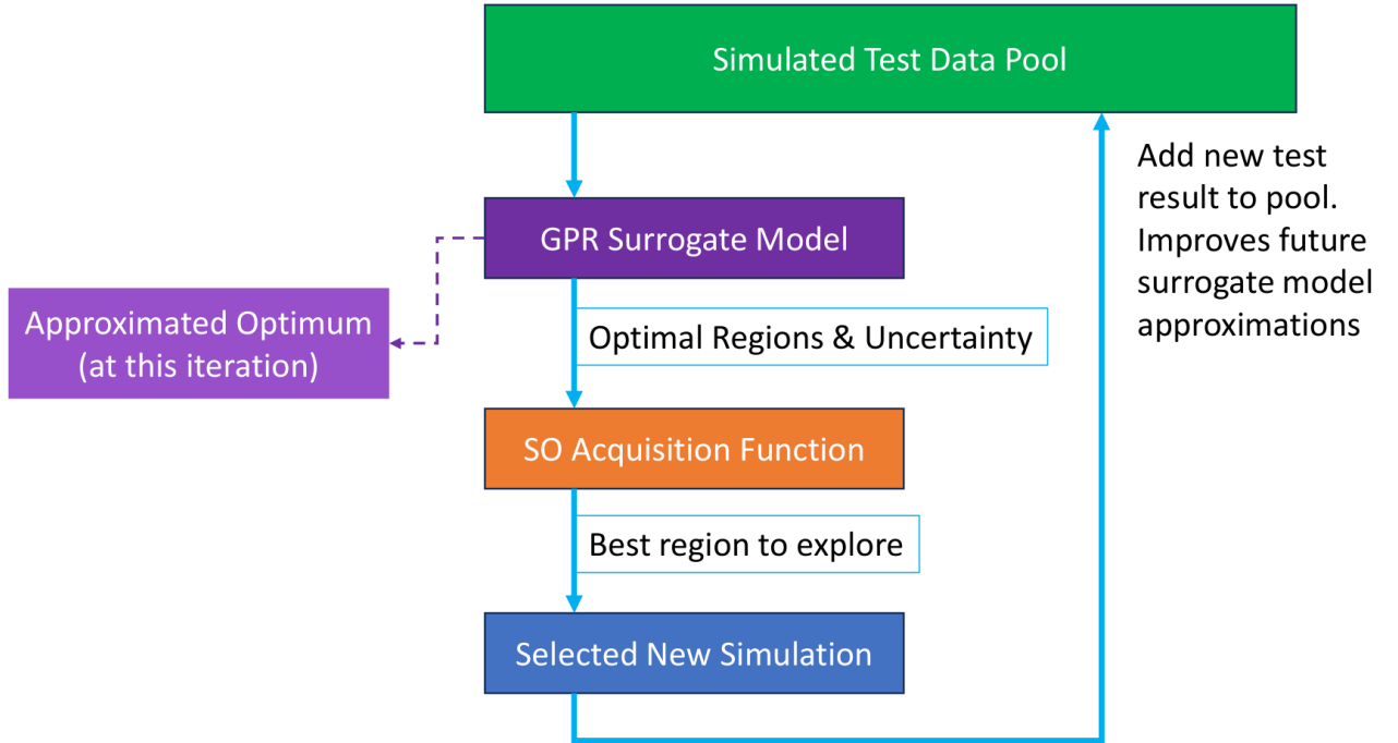
Figure B1: A simplified flowchart representing how simulation data is used and added to in the Single-Objective (SO) Bayesian Optimisation (BO) algorithm utilising Gaussian Process Regression (GPR).
