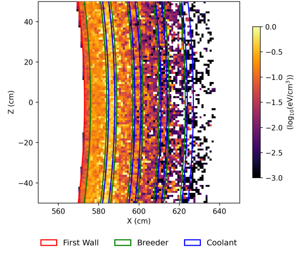
(b) Heating Energy Density ( \zeta = 0 )
