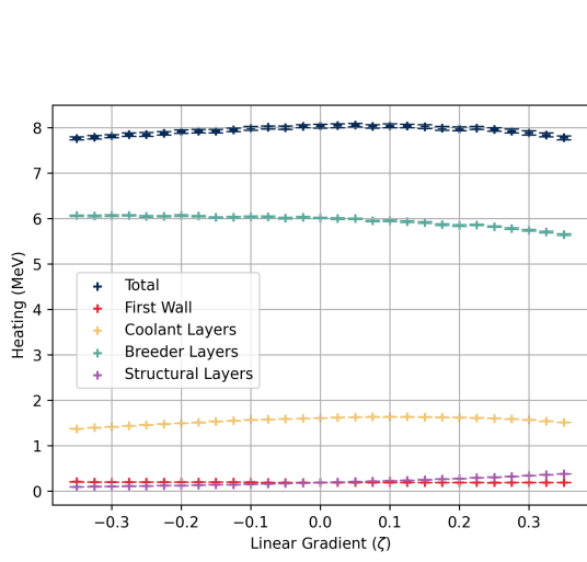
(a) Heating Energy vs \zeta
